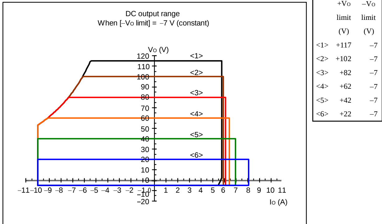
Figure 1-4. DC Output Range (When Negative Voltage Limiter Setting Is Fixed to -7 \text{ V} )
